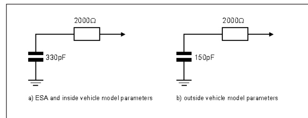
Figure 1: ESD Models
