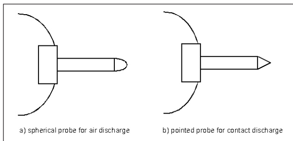
Figure 2: ESD Test Probes
